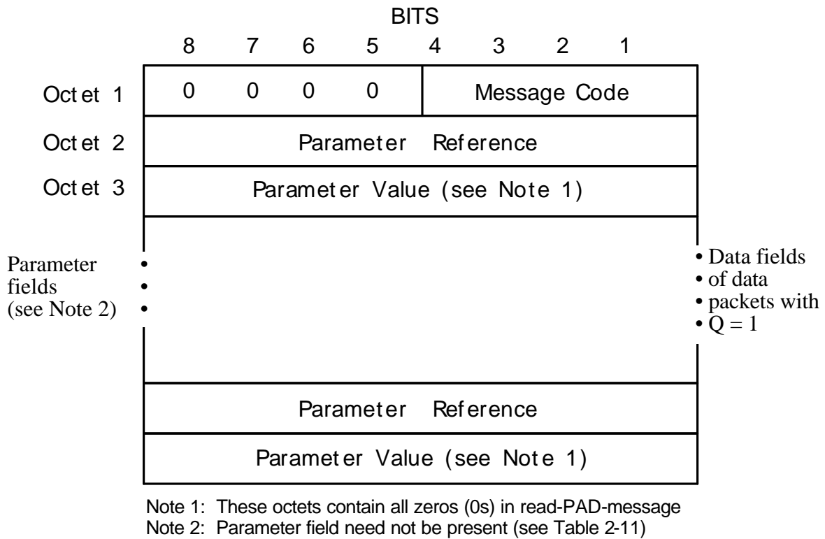
Figure 2-2 Set, Read, Set-And-Read And Parameter Indication Pad Message Format
