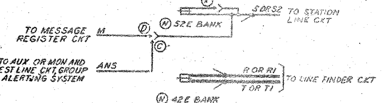
FIG. 3 BANK MULTIPLE NO. 701P OR 711P
