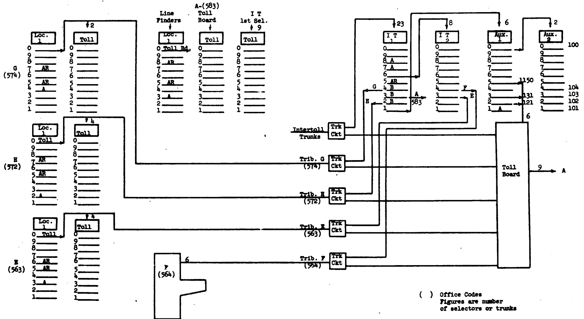
TOLL CENTER AREA - SWITCHING SCHEMATIC
