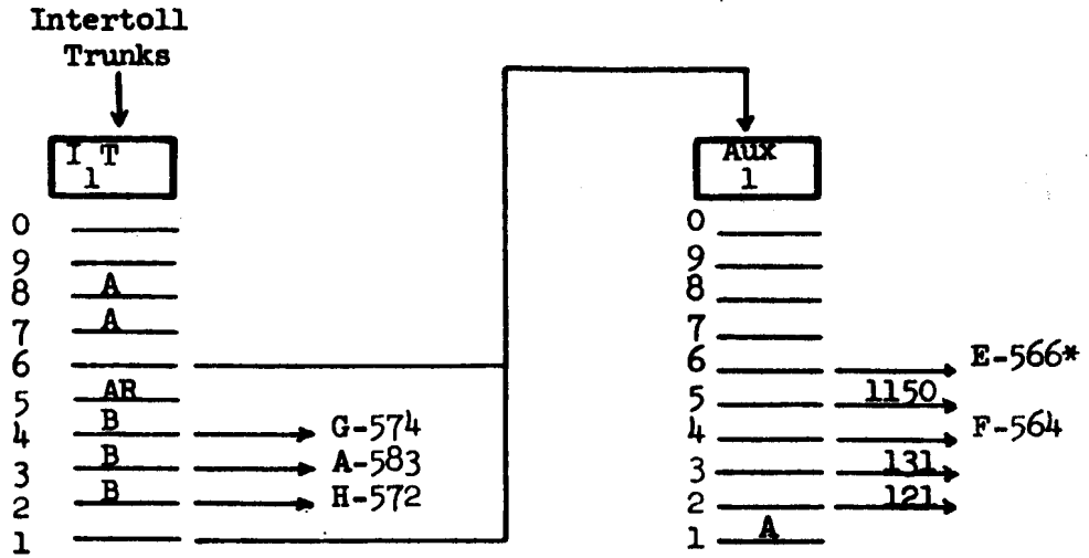
SCHEMATIC C
