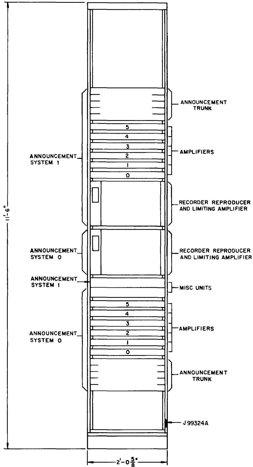
Fig. 1 — Announcement Frame — 5A Announcement System
