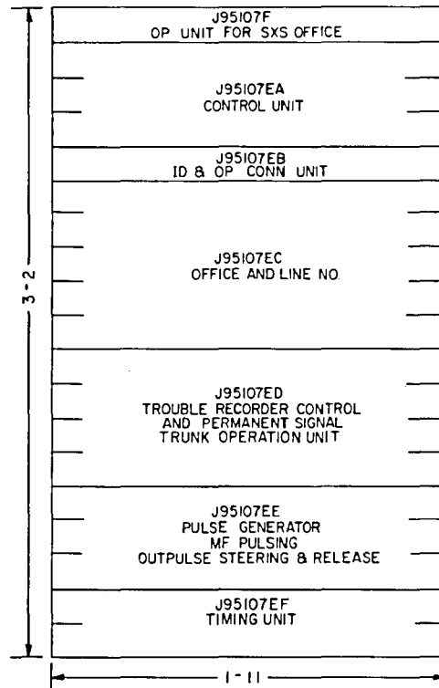
Fig 4—Outpulsor Unit Associated With 9-Foot Outpulsor Frame
