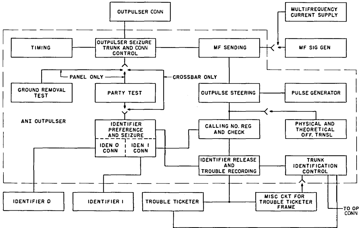
Fig 5—Typical System Block Diagram
