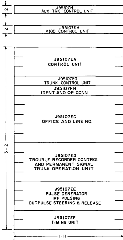
Fig 2—Outputpulser Unit Associated With 11-Foot 6-Inch Outputpulser Frame
