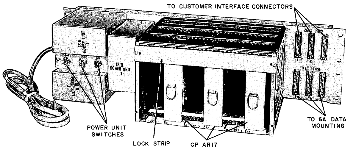
Fig. 1—Data Auxiliary Set 820E1, Front View
