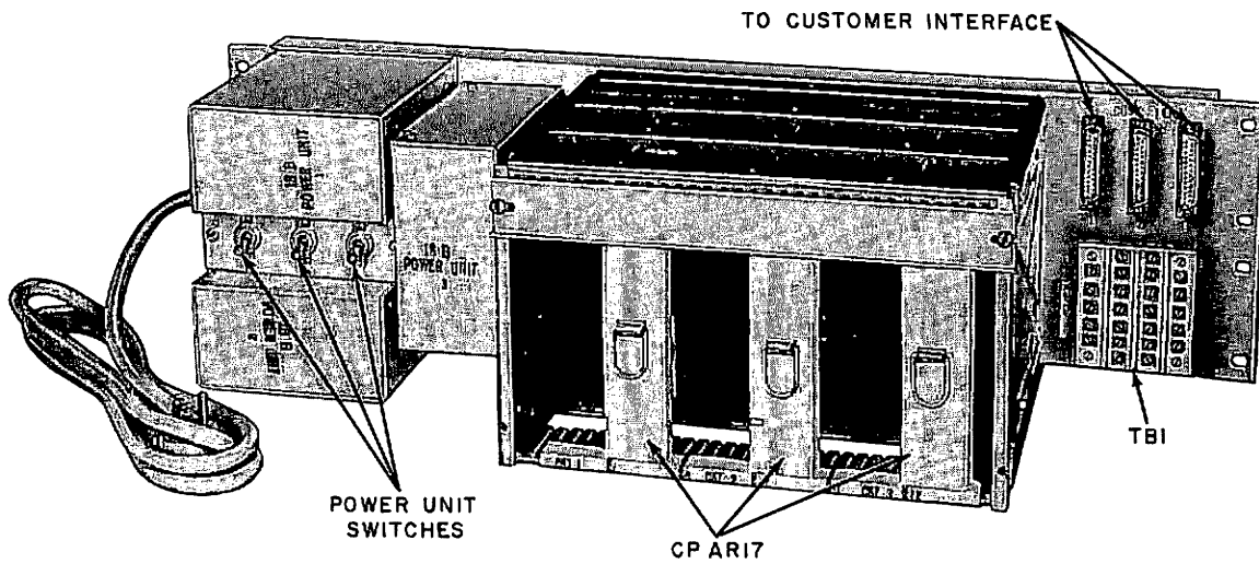
Fig. 2—Data Auxiliary Set 820E2, Front View
