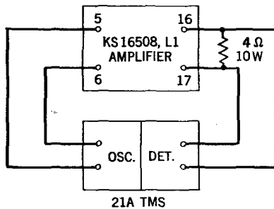
Fig. 5 - Gain-Frequency Test Setup for Record Channel
